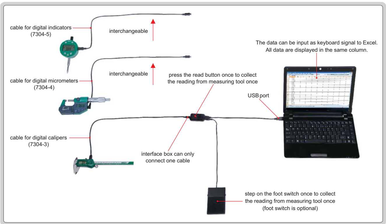
interface box 7304-1
