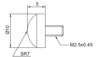
Spherical Point
