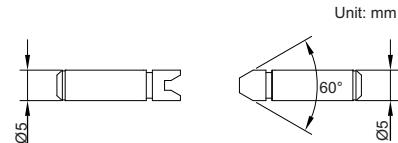
60° thread angle
